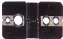
Front mounted die blades for stripping the inner insulation.
